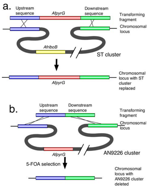
Figure 1. Two strategies for deletion of SM gene clusters. (a) The target strain is transformed with a fragment containing the A. fumigatus pyrG gene ( AfpypG ) flanked by two 2 kb sequences that are >50 kb apart in the genome, one upstream of the ST cluster and one downstream. The fragment is constructed by fusion PCR, 34,55 and the flanking fragments are amplified from genomic DNA using primers designed from genome sequence data. Upon transformation, homologous recombination results in the replacement of the entire ST cluster with AfpypG . AfriboB was previously inserted in the cluster, and replacement of the cluster with AfpypG results in removal of AfriboB causing riboflavin auxotrophy. (b) The AfpypG gene was previously inserted into the target cluster by transformation. The transforming fragment is composed of two sequences: one from just upstream of the cluster and the other from just downstream of the cluster. They are amplified from genomic DNA and joined by fusion PCR. Upon transformation, homologous recombination results in excision of the target cluster including AfpypG . Transformants in which AfpypG has been excised are selected on 5-FOA. AfpypG can be subsequently reused as a selectable marker.
