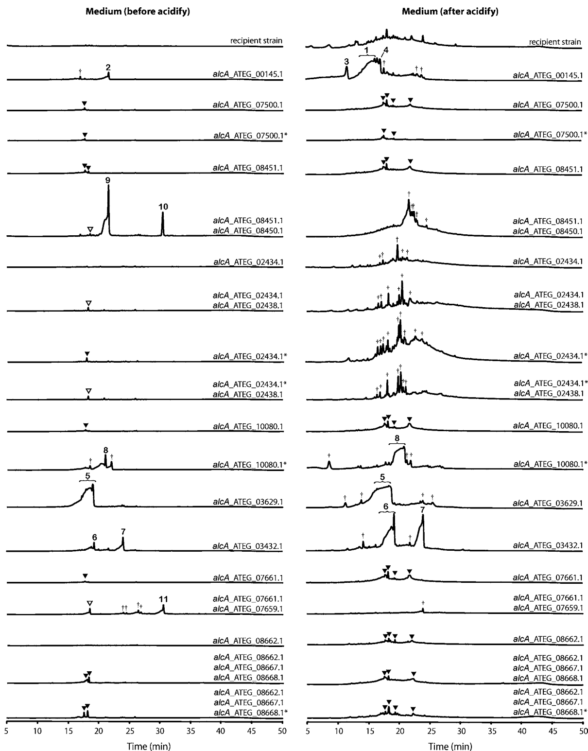
Figure 5. Total scan HPLC profiles of metabolites extracted from the culture medium before or after acidification of A. nidulans strains expressing A. terreus genes under the control of alca (p). The genes expressed are listed above each trace. The numbering of the peaks corresponds to compounds shown in Figure 4. Peaks that are also present in other strains are marked by a black triangle (▼) and are considered not to be specific to the expressed genes. Peaks that are specifically present in induced strains but are not structurally elucidated due to low yield or pool stability are marked with a dagger (†). ▽: Lumichrome, a degraded product from riboflavin. *: Transferred genes with a revised start site.
