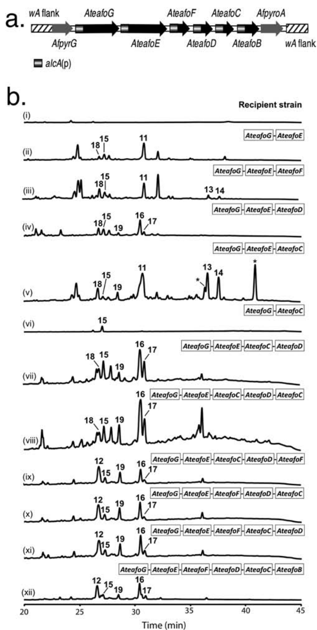
Figure 7. The A. terreus asperfuranone ( Atefo ) gene cluster assembled in A. nidulans with each gene placed under control of the alcA promoter. Total scan HPLC profiles of metabolites extracted from the culture media of A. nidulans strains expressing A. terreus af o cluster genes under the control of alcA(p) . The numbering of the peaks corresponds to compounds shown in Figure 8. The Atefo genes expressed are listed above each trace, and (i) is the trace for the control strain. * denotes unstable metabolites that have different chromophores from those compounds identified in this study.
