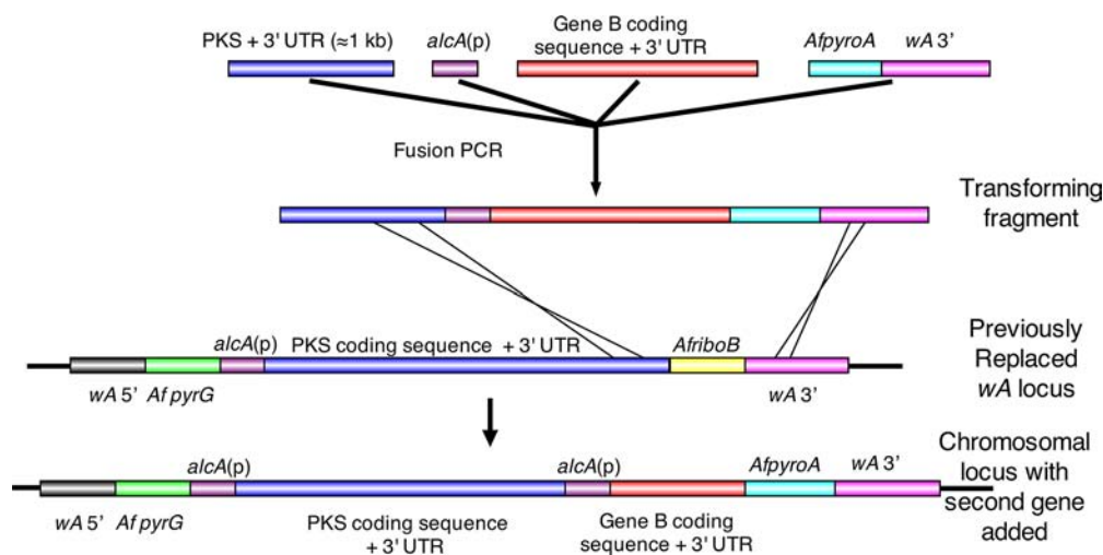
Figure 3. Transferral of additional genes with marker recycling. Using a four piece fusion PCR, we create a transforming fragment containing \approx 1000 bp from the C-terminus of the PKS already inserted ( \approx 900 bp of coding sequence plus \approx 100 bp of 3' untranslated region), alcA(p) , the coding sequence of the gene of interest plus \approx 100 bp of 3' untranslated region, AfpyroA , a selectable marker, 34 and \approx 1000 bp of wA downstream sequence. Transformation with this fragment inserts the gene, under the control of alcA(p) , and it evicts AfriboB , allowing it to be used as a selectable marker for the next transformation. In principle, recombination between alcA(p) on the transforming fragment and alcA(p) upstream of the PKS could cause deletion of the PKS, but in practice, this event did not occur frequently enough to hinder progress. To add a third gene, the process is repeated except that AfriboB is used as a selectable marker, and AfpyroA is excised upon transformation. The process can be repeated over and over.
